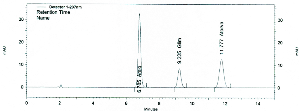
Figure 3.13. Profiles of each concentration point (0.5, 1, and 1.5 mg/ml, respectively) of amlodipine, glimepiride and atorvastatin. Peaks are directly correlated to concentration.
